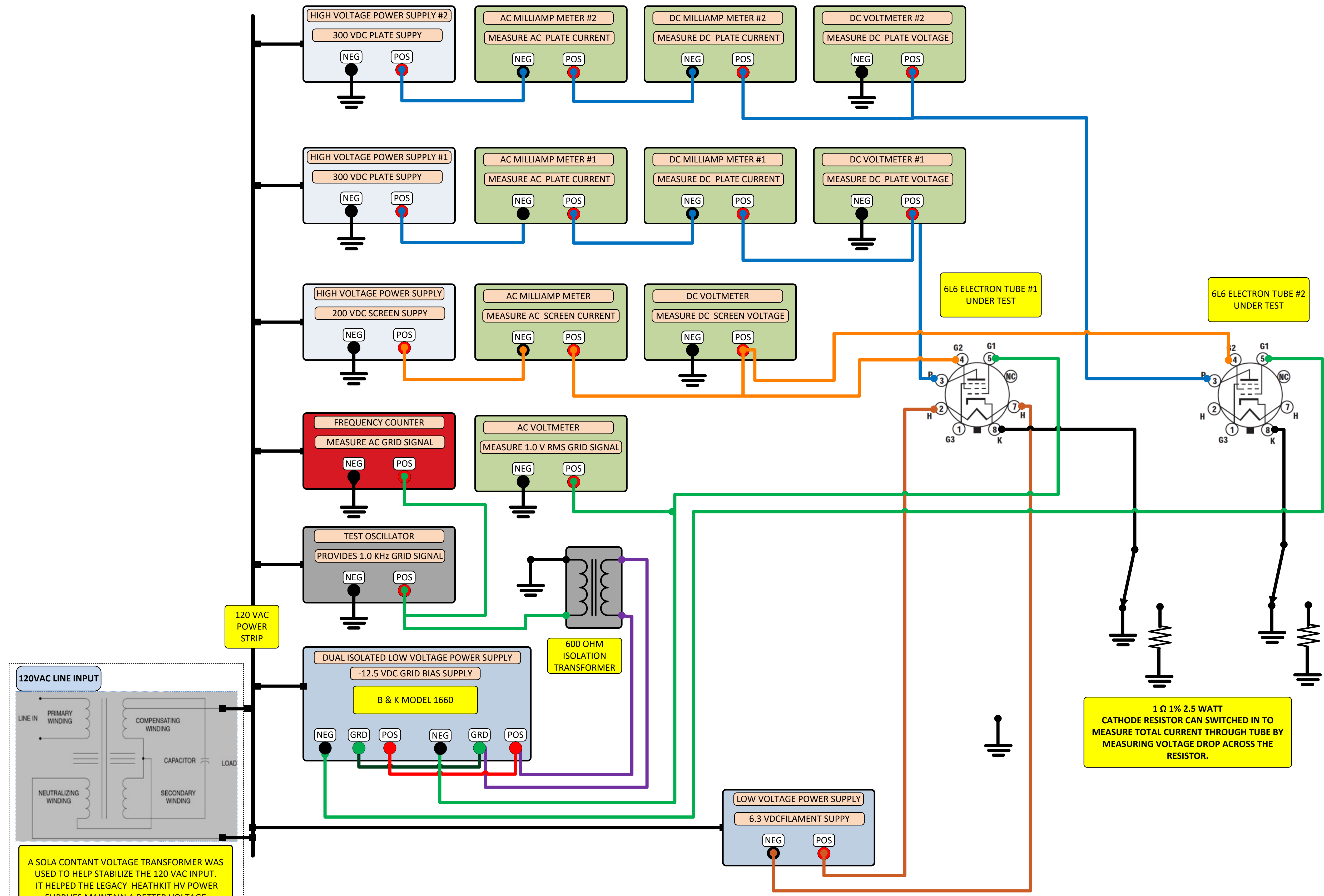
FUNCTIONAL SCHEMATIC SET-UP TO ALLOW THE TESTING OF TWO TUBES SIMULTANEOUSLY
